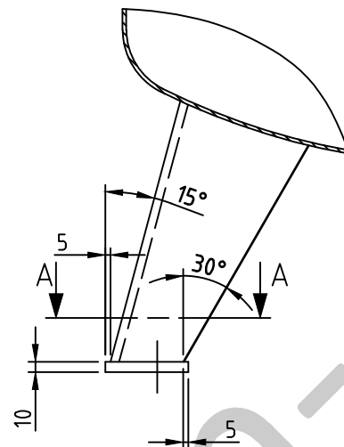
Detail X
